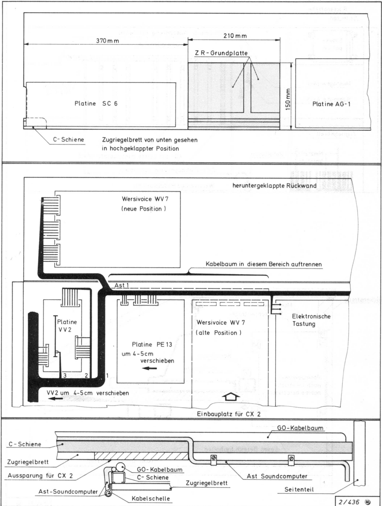
Abb. 27e: CX 2 in W 1 T COMBO
